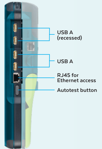
MAINFRAME RIGHT SIDE
