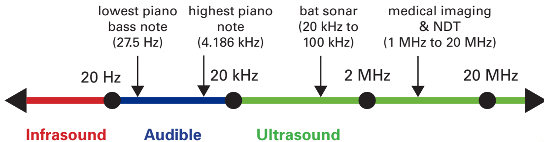
Approximate frequencies of common sounds.
